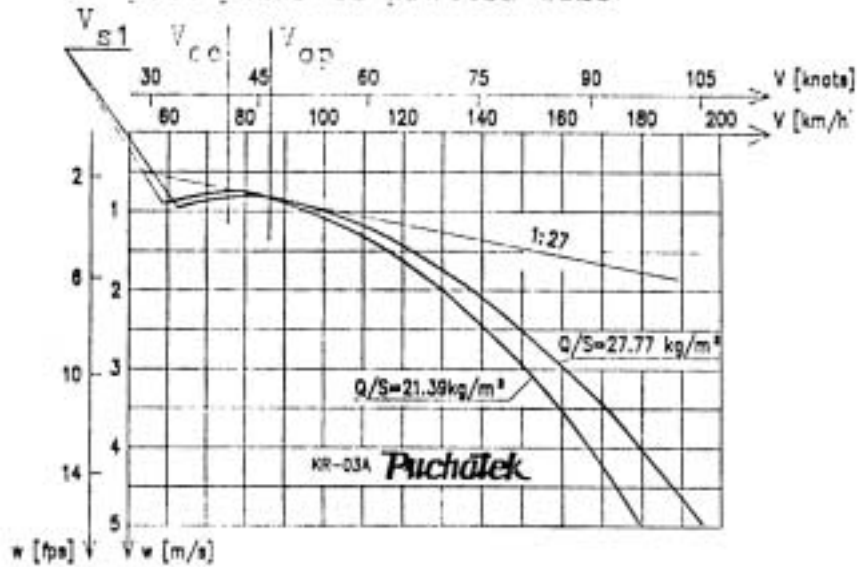
Speed polar of KR-03A "Puchatek" glider
